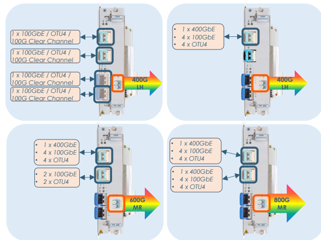
Figure 1: Multiple operating modes of PM 800FR04
