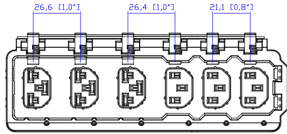
VIEW B
